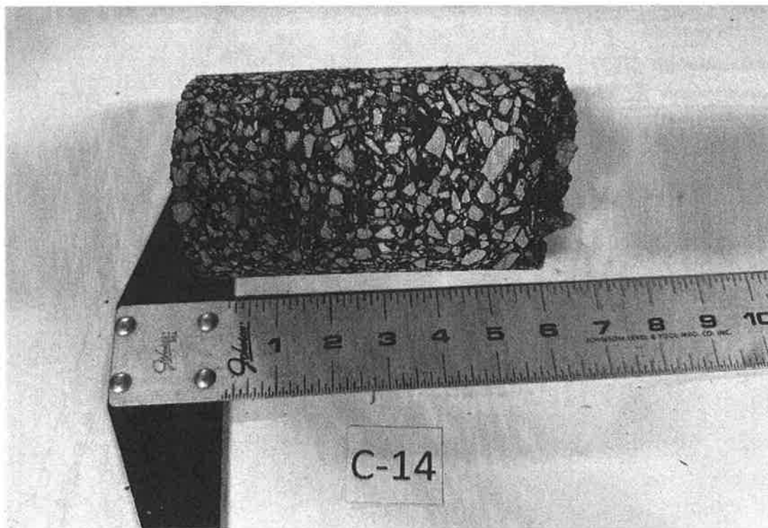
Pavement Core C-14: Kane County Judicial Center
