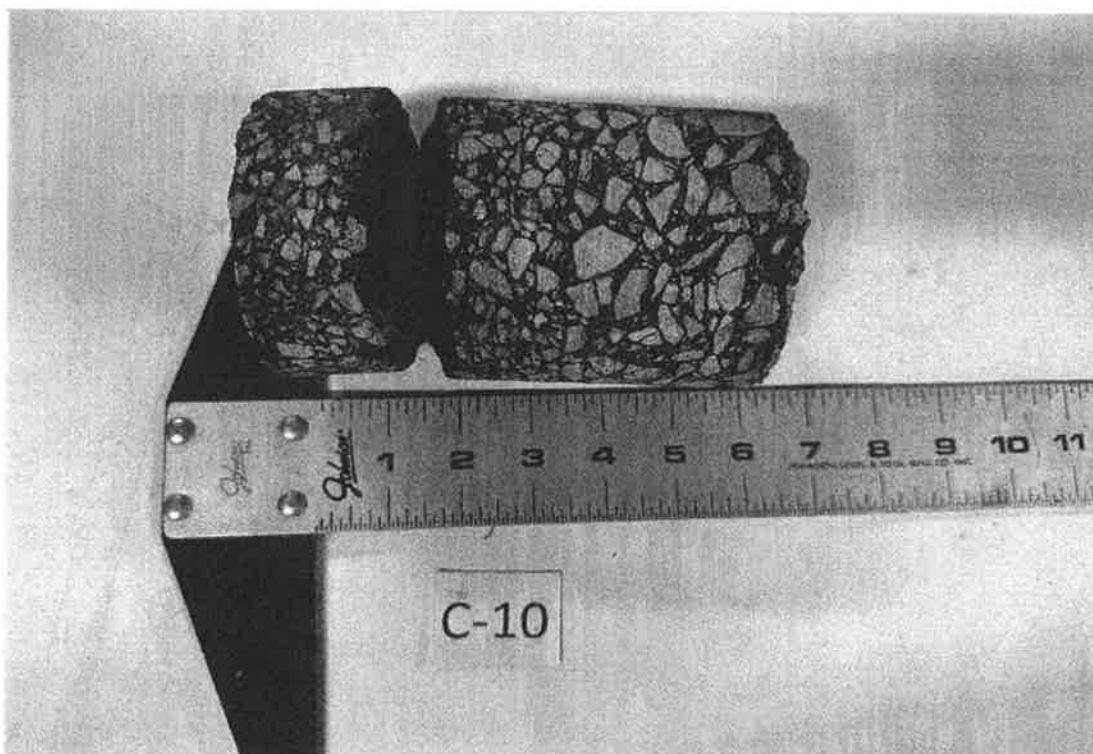
Pavement Core C-10: Kane County Judicial Center
