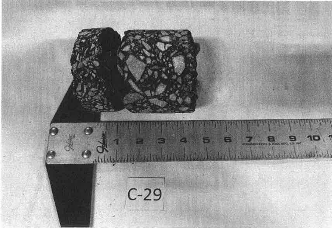
Pavement Core C-29: Kane County Judicial Center
