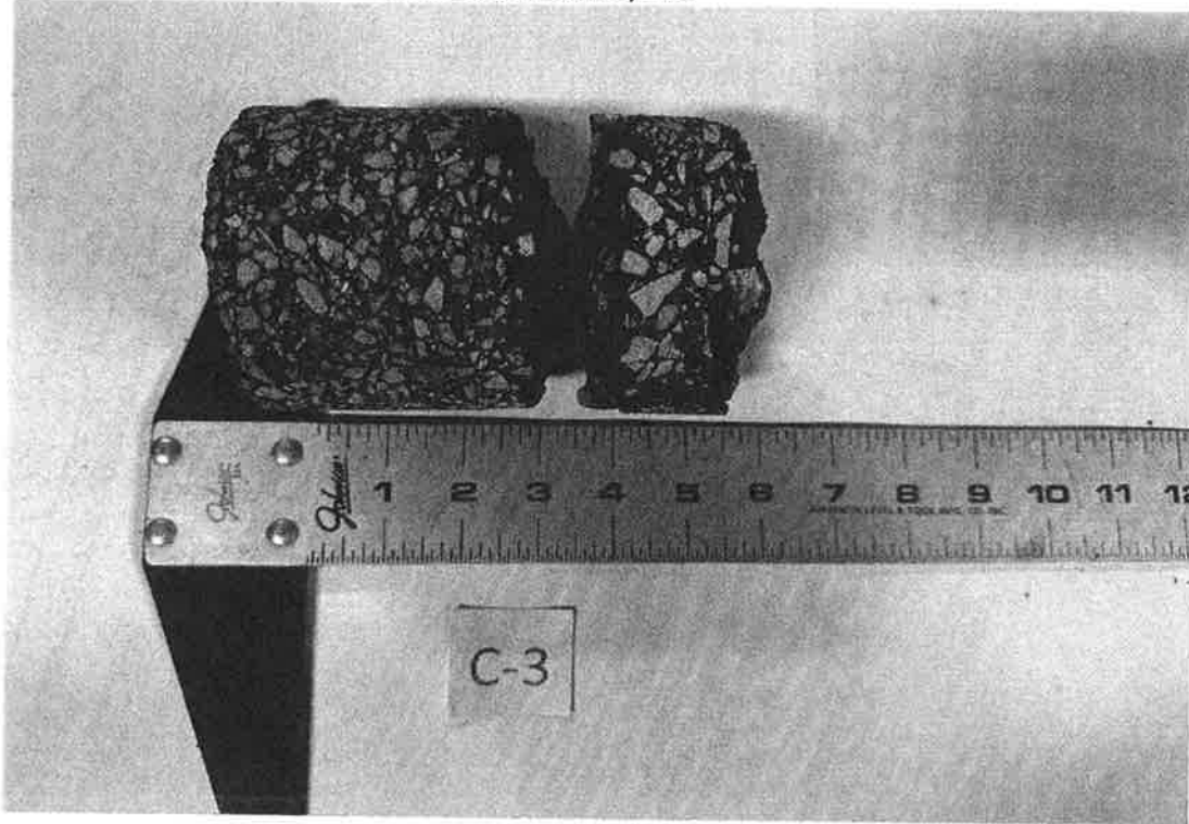
Pavement Core C-3: Kane County Judicial Center
