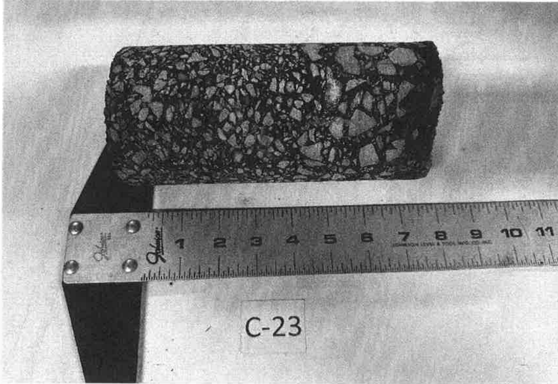
Pavement Core C-23: Kane County Judicial Center
