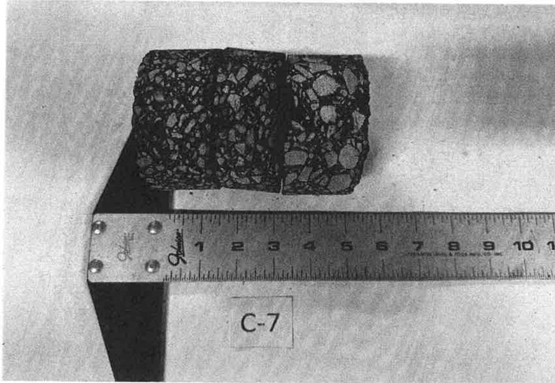
Pavement Core C-7: Kane County Judicial Center
