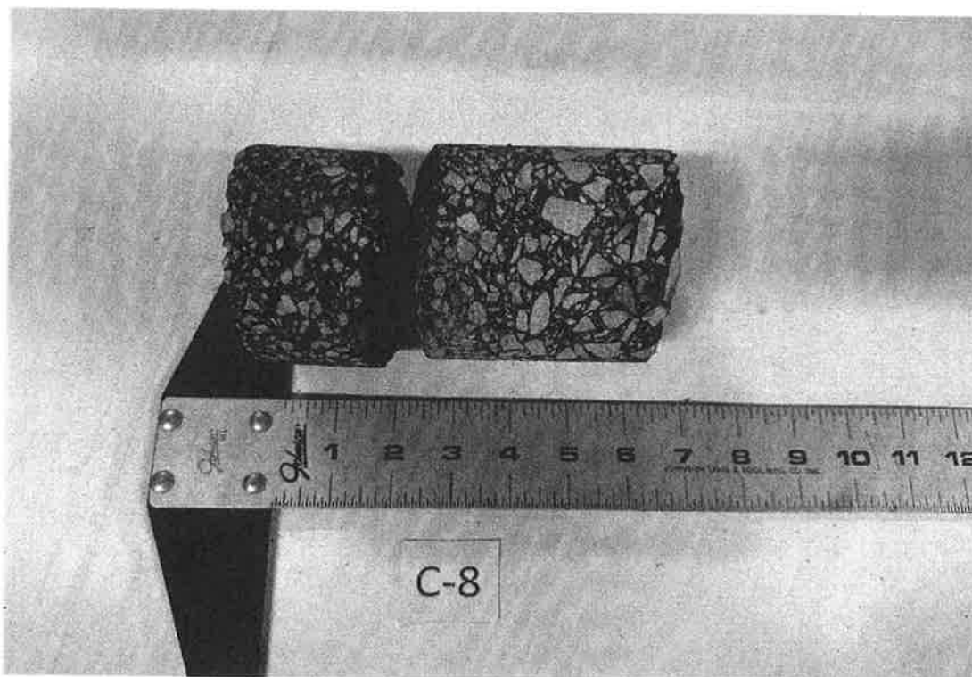
Pavement Core C-8: Kane County Judicial Center
