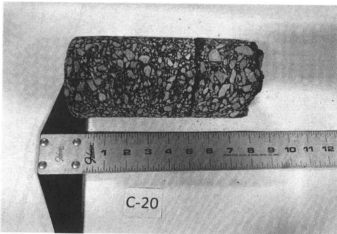
Pavement Core C-20: Kane County Judicial Center
