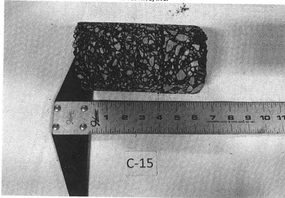
Pavement Core C-15: Kane County Judicial Center
