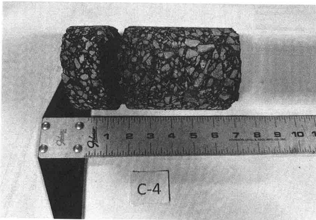
Pavement Core C-4: Kane County Judicial Center
