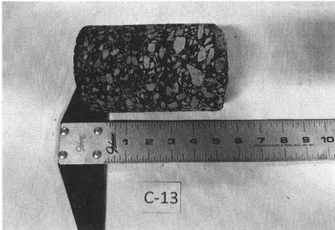
Pavement Core C-13: Kane County Judicial Center
