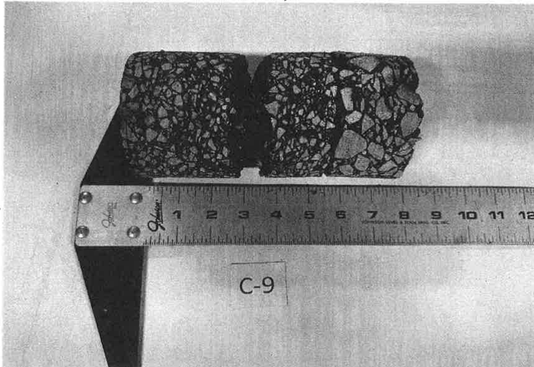
Pavement Core C-9: Kane County Judicial Center
