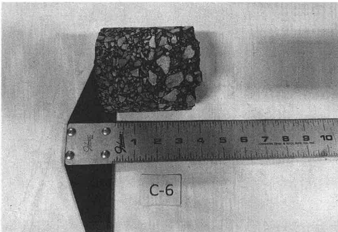
Pavement Core C-6: Kane County Judicial Center
