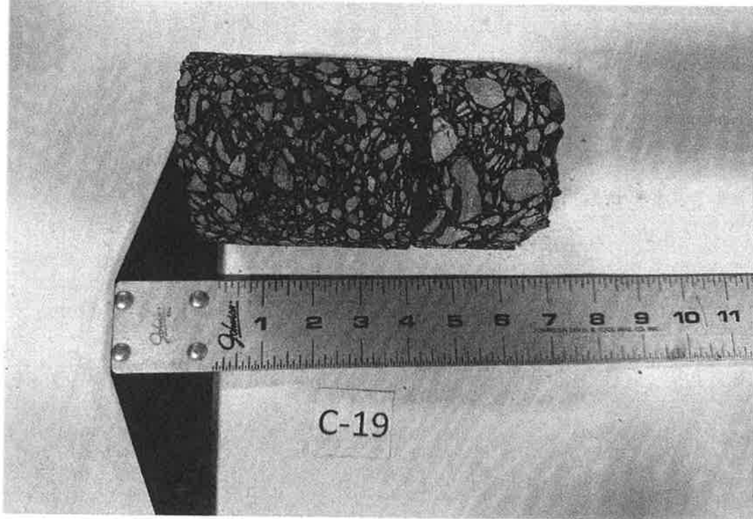
Pavement Core C-19: Kane County Judicial Center
