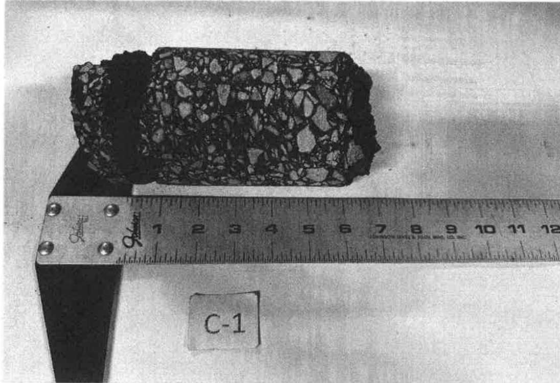
Pavement Core C-1: Kane County Judicial Center
