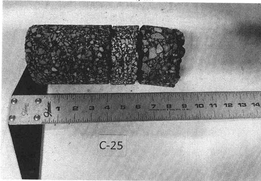
Pavement Core C-25: Kane County Judicial Center
